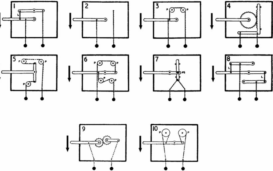
Diagrams of open boxes (P = pulley wheel: PS = pin and slot: L= solid link)
