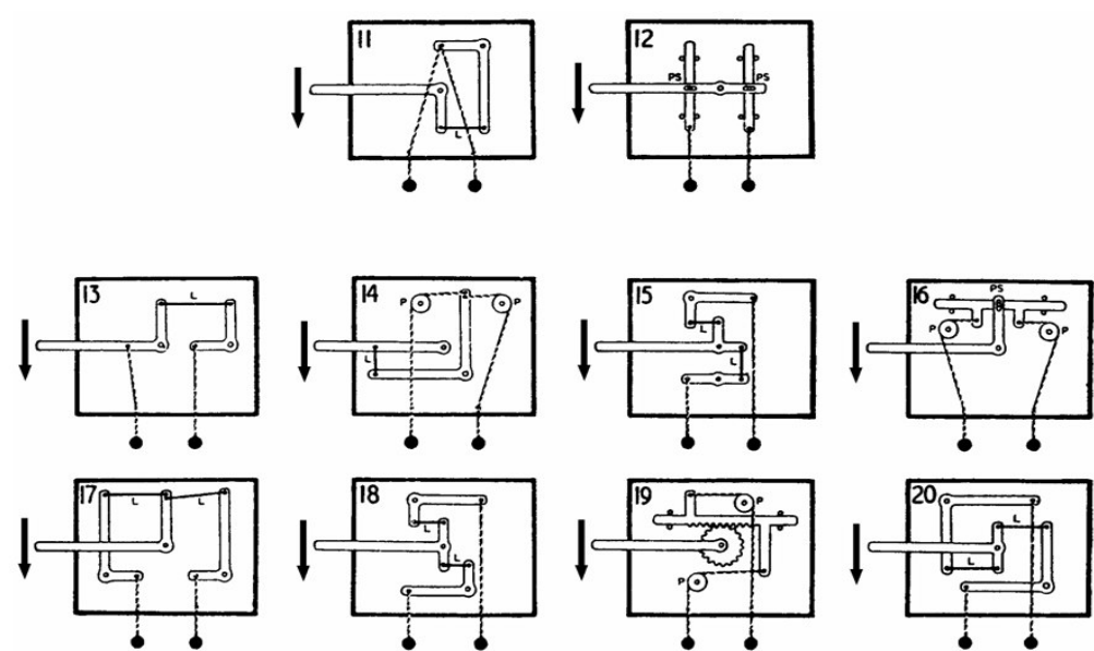
Diagrams of open boxes (P = pulley wheel: PS = pin and slot: L= solid link)
